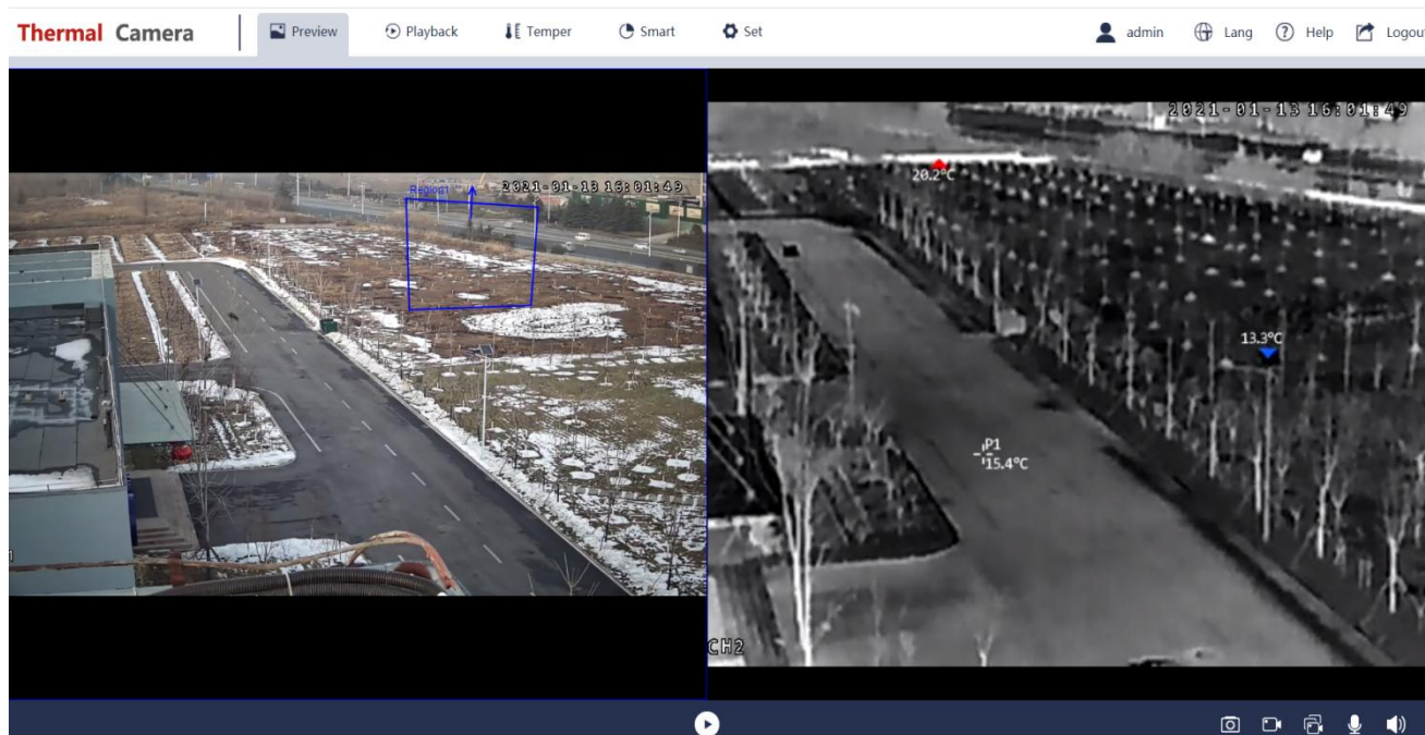
Figure 2.1 Preview Interface
